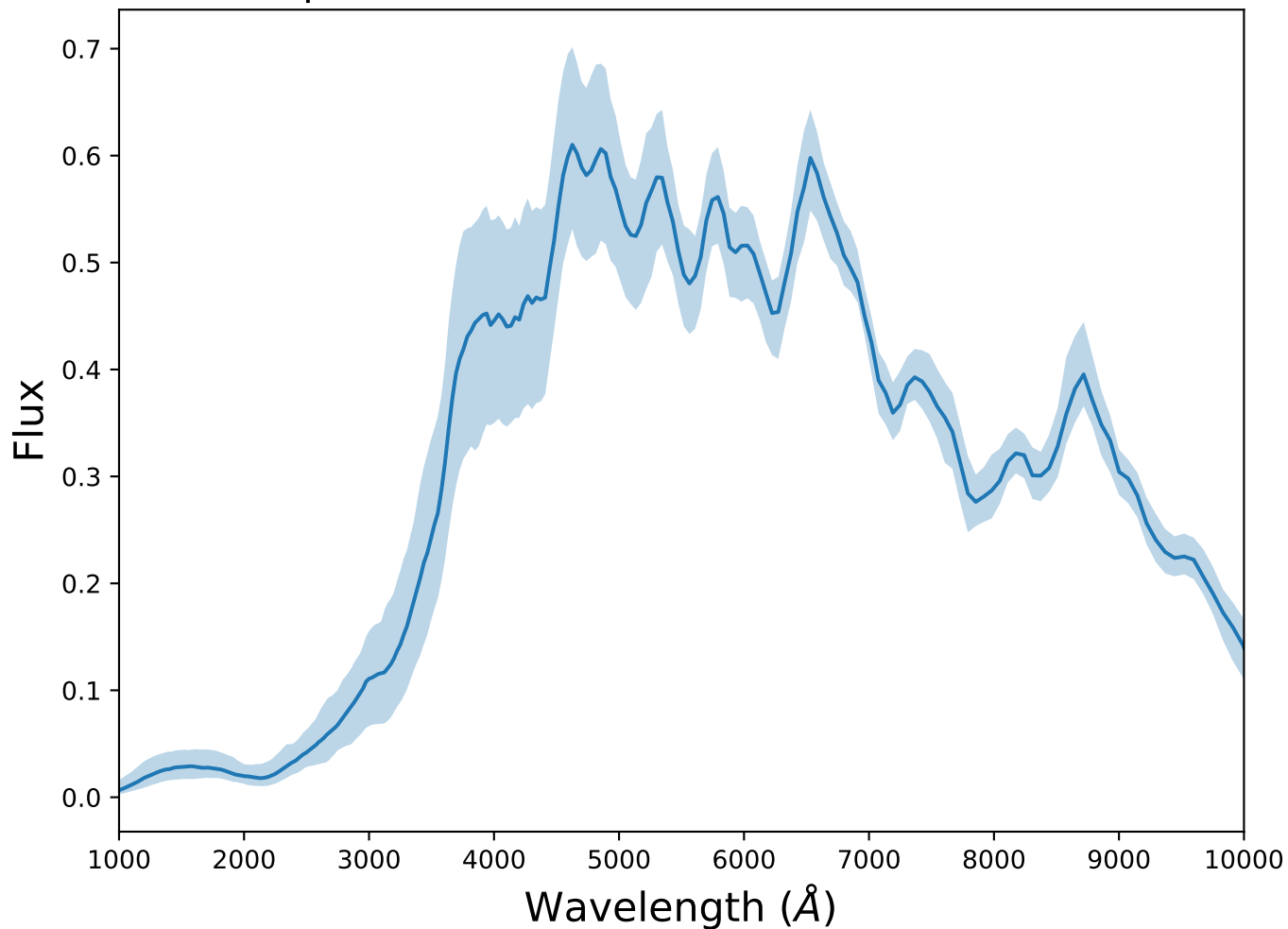
Spectrum 1 for transient ILOT at z=0.75
